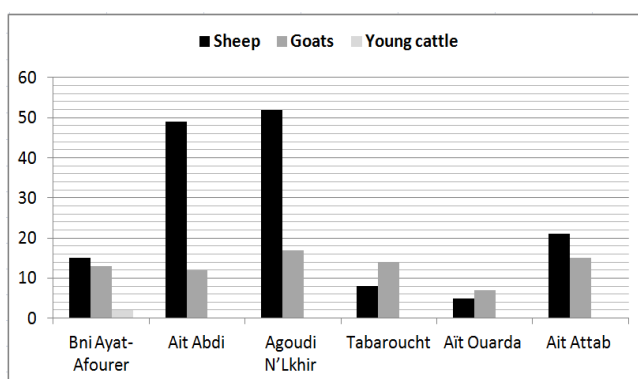
Figure 4. The number of domestic animals killed by Canis spp. in six regions belonging to the central High Atlas Mountains, Morocco, in 2019 – 2021.
