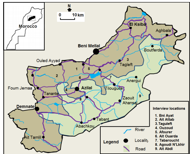
Figure 1. The central High Atlas Mountains, showing the main rivers, roads, localities, and the villages where the surveys were carried out. The rectangle on the inset indicates the location of the study area in Morocco.
